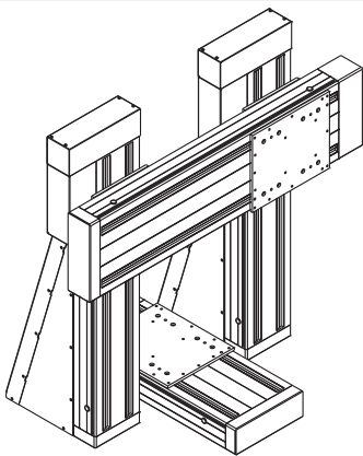
3-axis portal configuration
