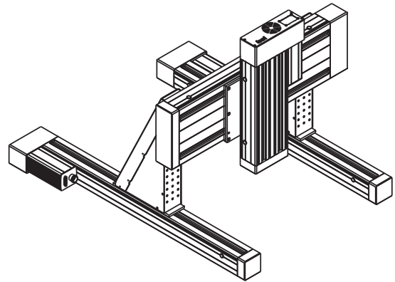
3-axis flatbed configuration
